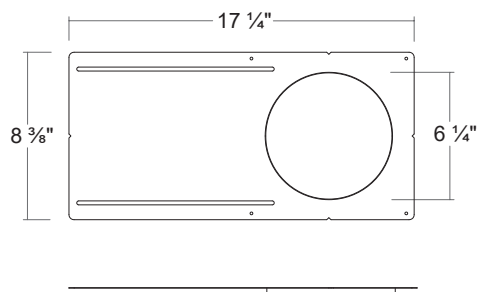
LRP60 6" Mounting Plate / Round
